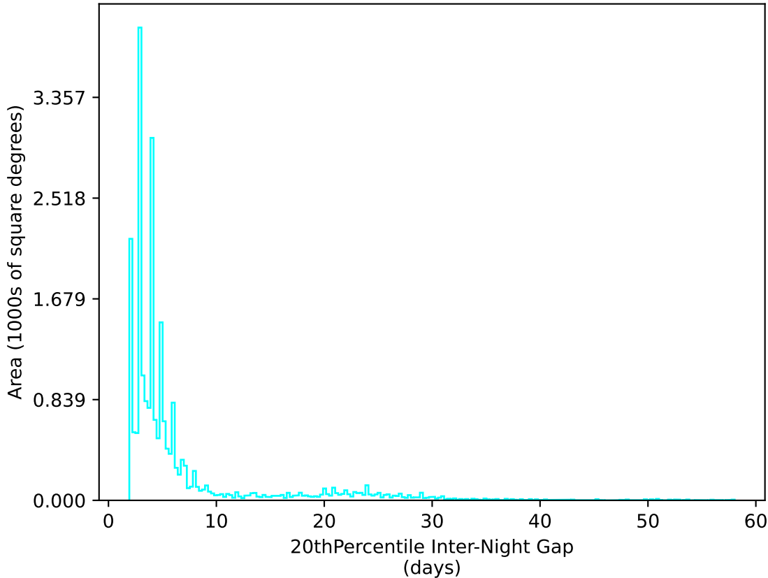
no_magell_roll_v3.4_10yrs All sky u band: 20thPercentile Inter-Night Gap
