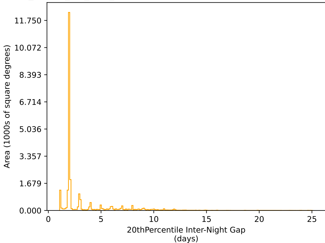
no_magell_roll_v3.4_10yrs All sky r band: 20thPercentile Inter-Night Gap
