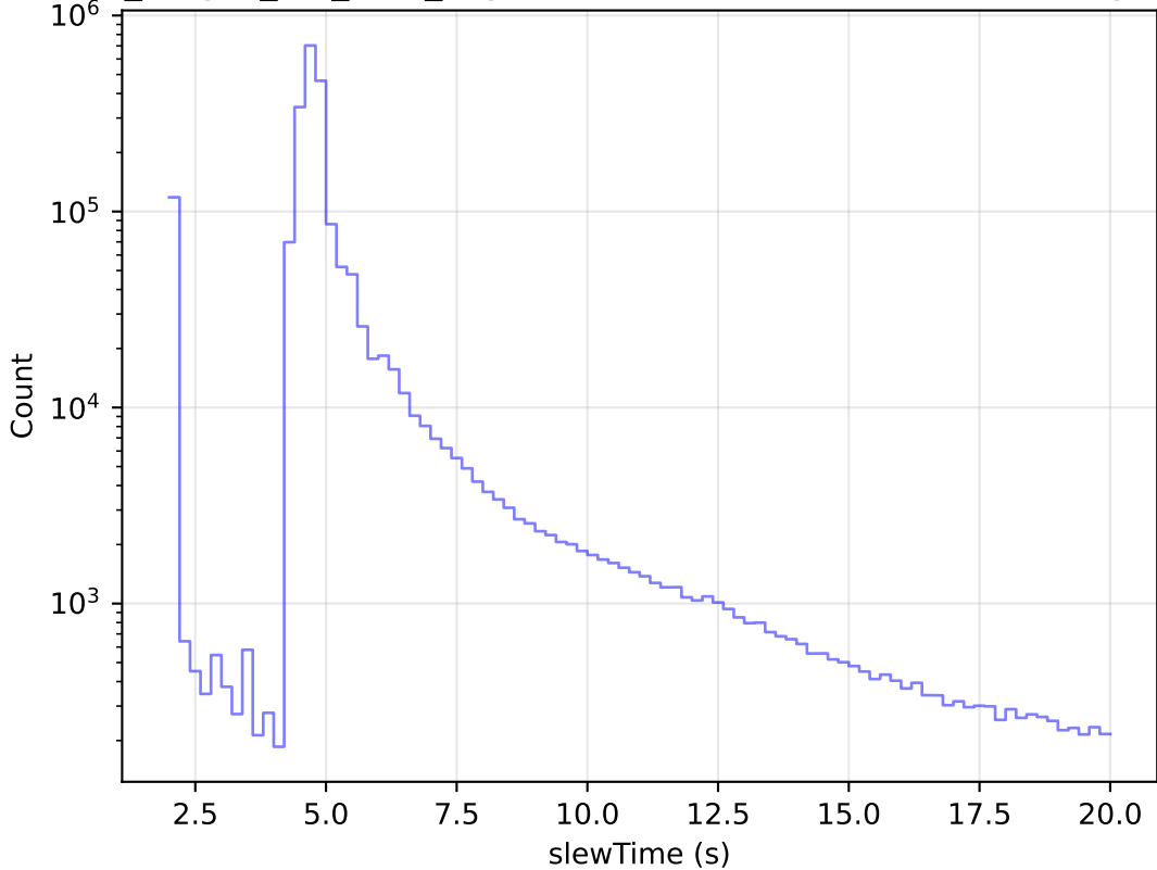
no_magell_roll_v3.4_10yrs All visits: Zoom Slew Time Histogram
