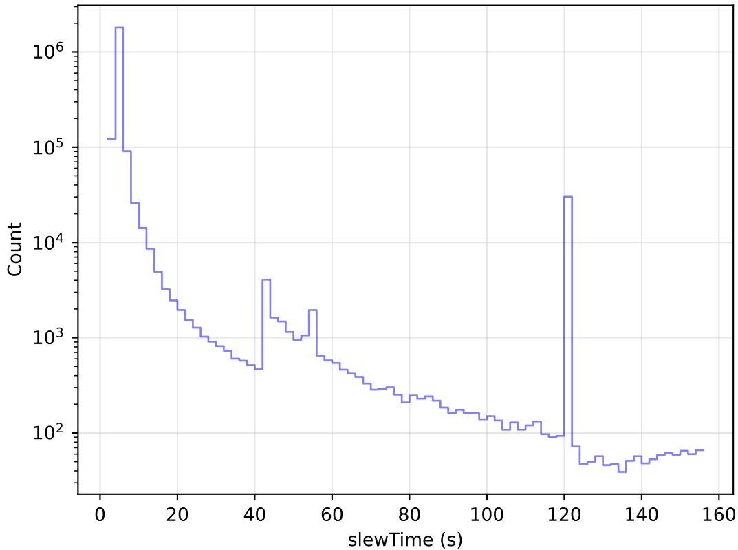
no_magell_roll_v3.4_10yrs All visits: Slew Time Histogram
