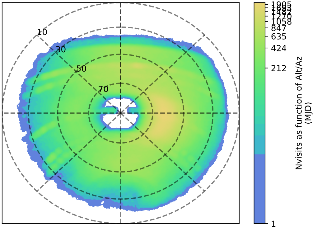
no_magell_roll_v3.4_10yrs y: Nvisits as function of Alt/Az
