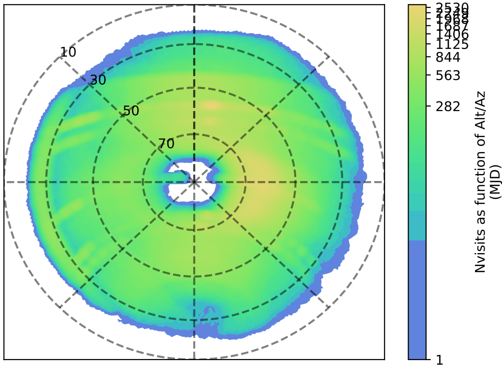
no_magell_roll_v3.4_10yrs r: Nvisits as function of Alt/Az
