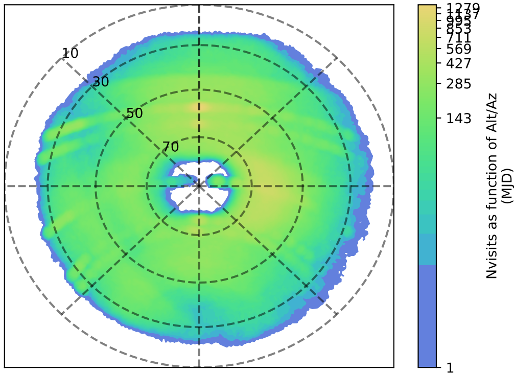
no_magell_roll_v3.4_10yrs g: Nvisits as function of Alt/Az
