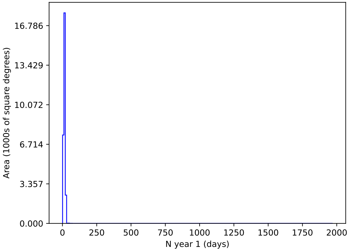
no_magell_roll_v3.4_10yrs z and night < 365: N year 1
