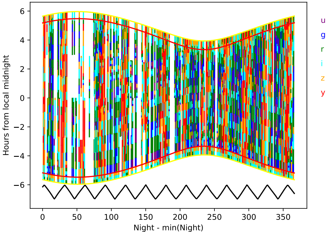
no_magell_roll_v3.4_10yrs year 9-10: Hourglass
