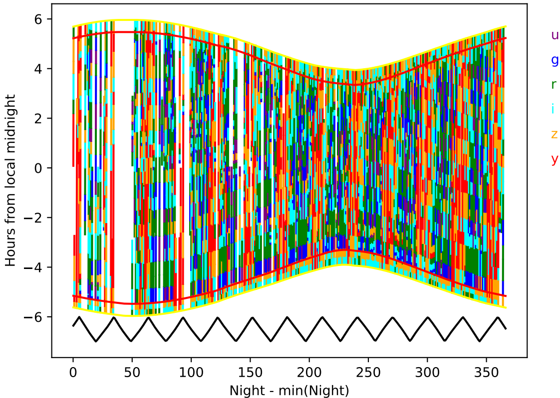
no_magell_roll_v3.4_10yrs year 6-7: Hourglass
