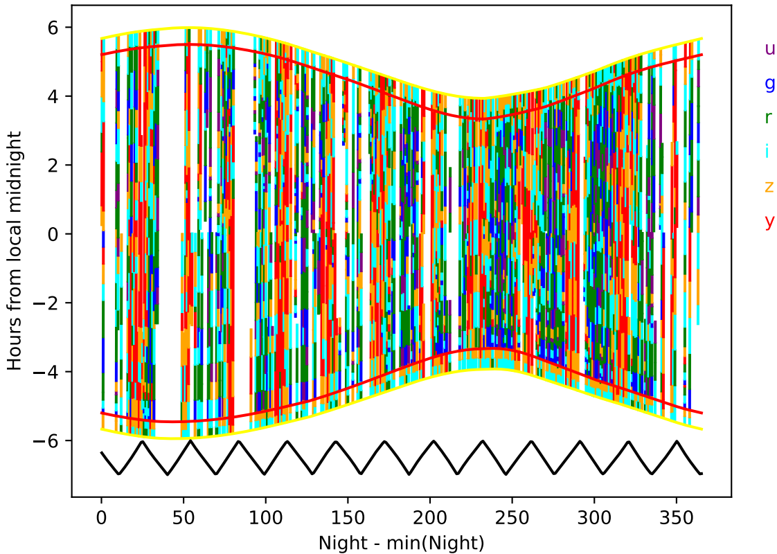
no_magell_roll_v3.4_10yrs year 4-5: Hourglass
