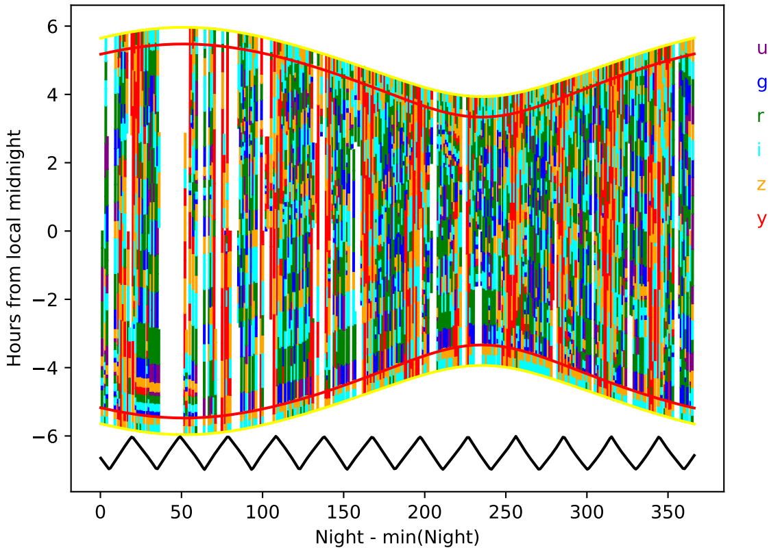
no_magell_roll_v3.4_10yrs year 2-3: Hourglass
