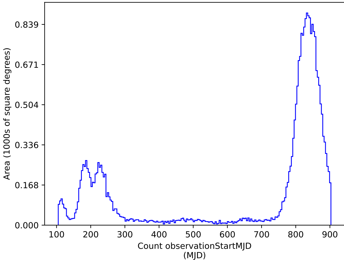
no_magell_roll_v3.4_10yrs : Count observationStartMJD
