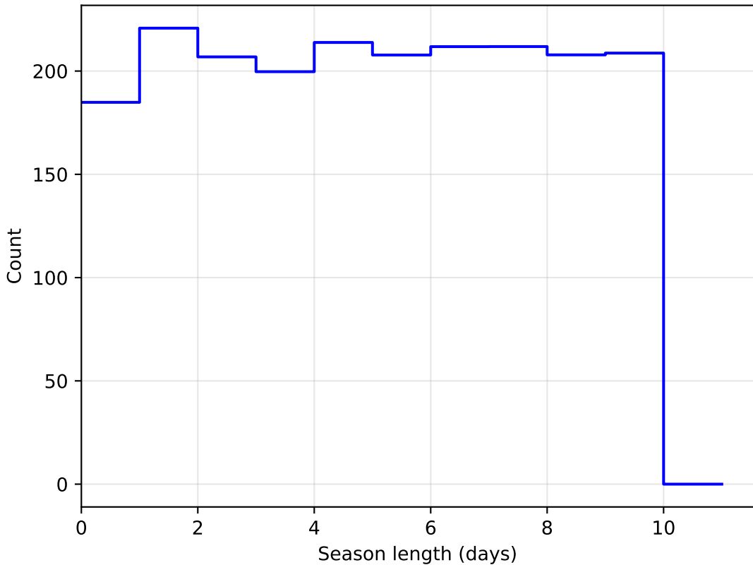
no_magell_roll_v3.4_10yrs DD:ELAISS1 all bands: SeasonLength
