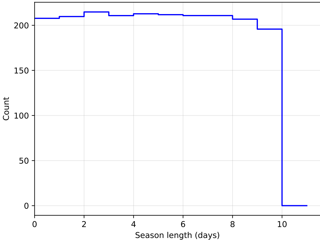
no_magell_roll_v3.4_10yrs DD:EDFS all bands: SeasonLength
