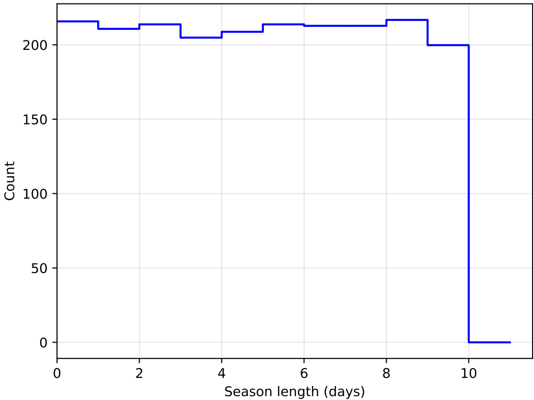
no_magell_roll_v3.4_10yrs DD:ECDFS all bands: SeasonLength
