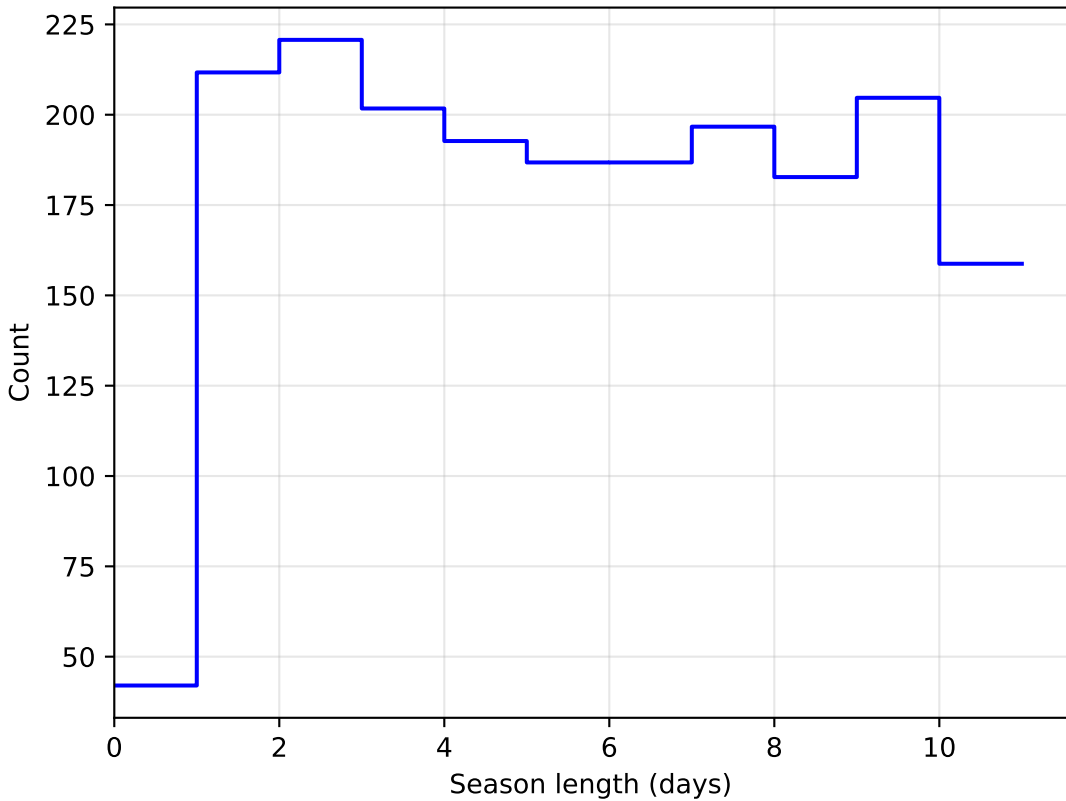
no_magell_roll_v3.4_10yrs DD: COSMOS all bands: SeasonLength
