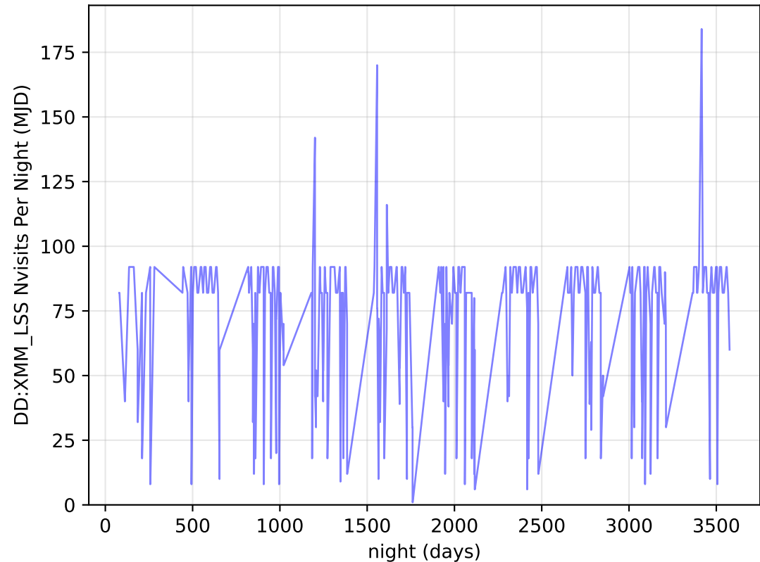
no_magell_roll_v3.4_10yrs all bands: DD:XMM_LSS Nvisits Per Night
