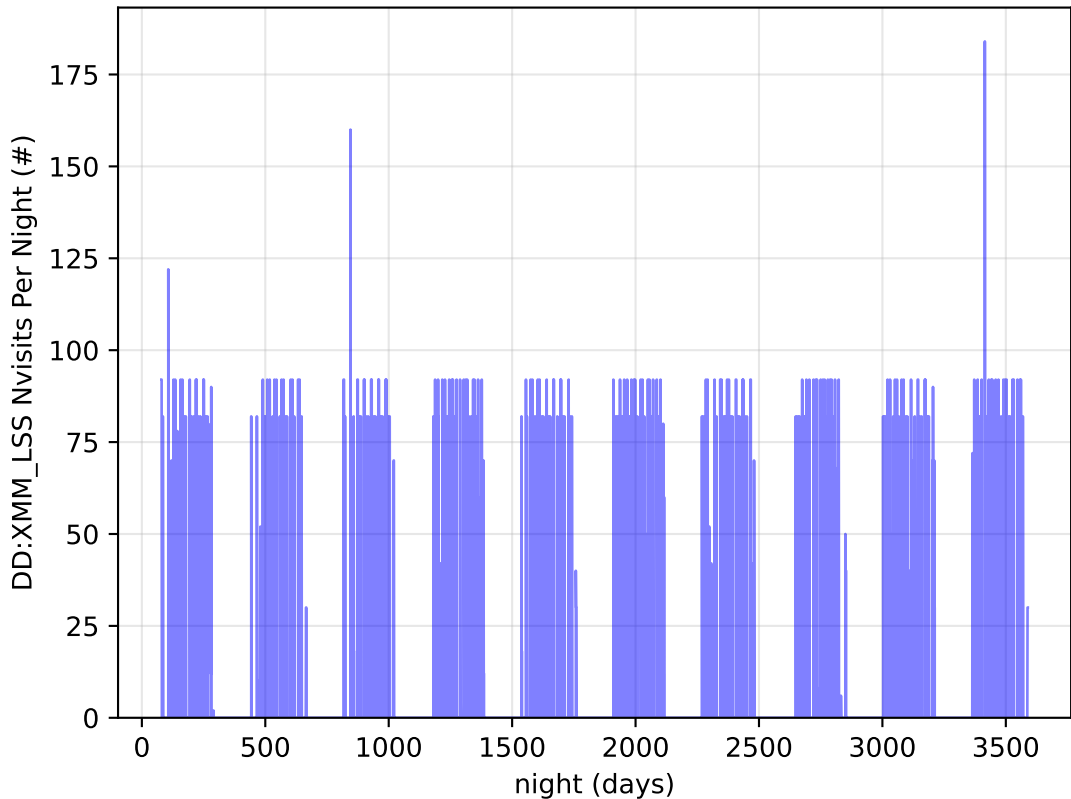
no_magell_roll_v3.4_10yrs all bands: DD:XMM_LSS Nvisits Per Night
