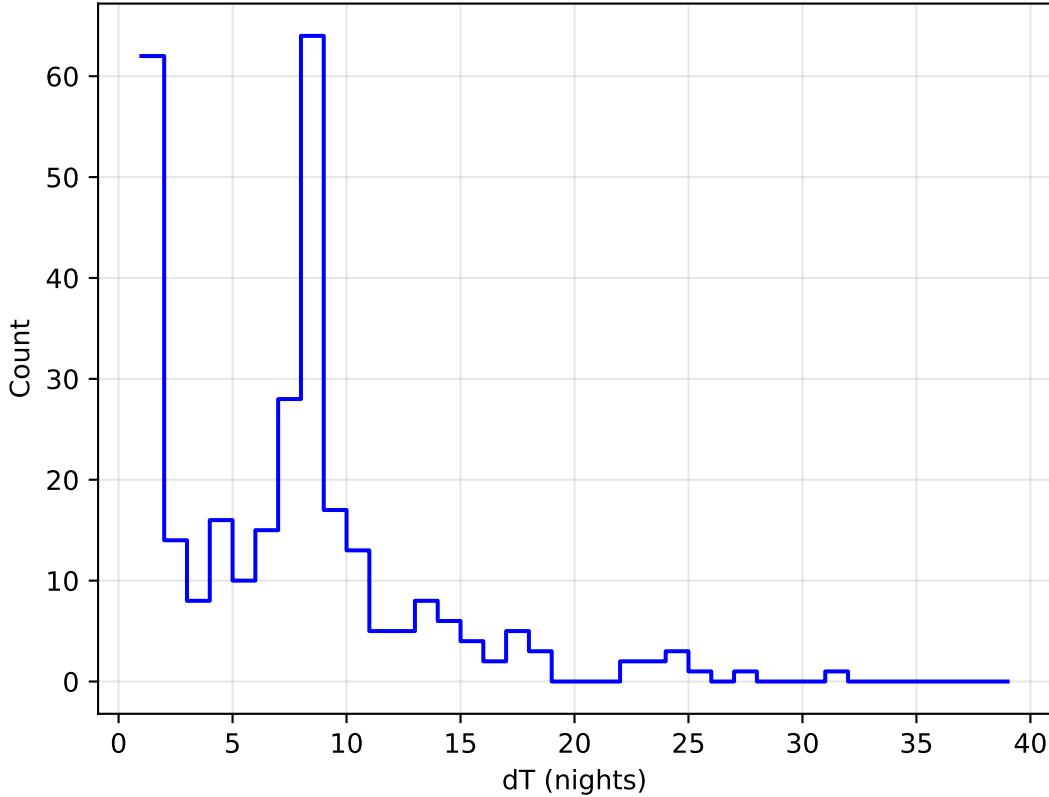
no_magell_roll_v3.4_10yrs all bands: DD:XMM_LSS Delta Nights Histogram
