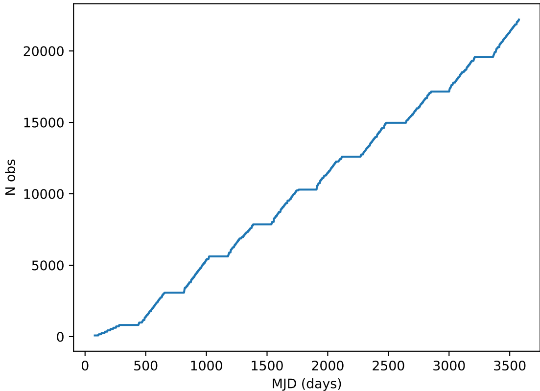
no_magell_roll_v3.4_10yrs all bands: DD:XMM_LSS Cumulative NVisits
