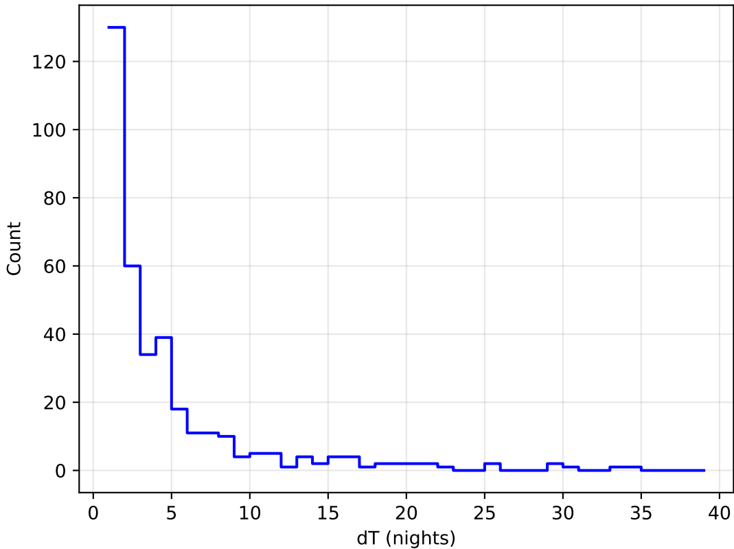
no_magell_roll_v3.4_10yrs all bands: DD:WFD Delta Nights Histogram
