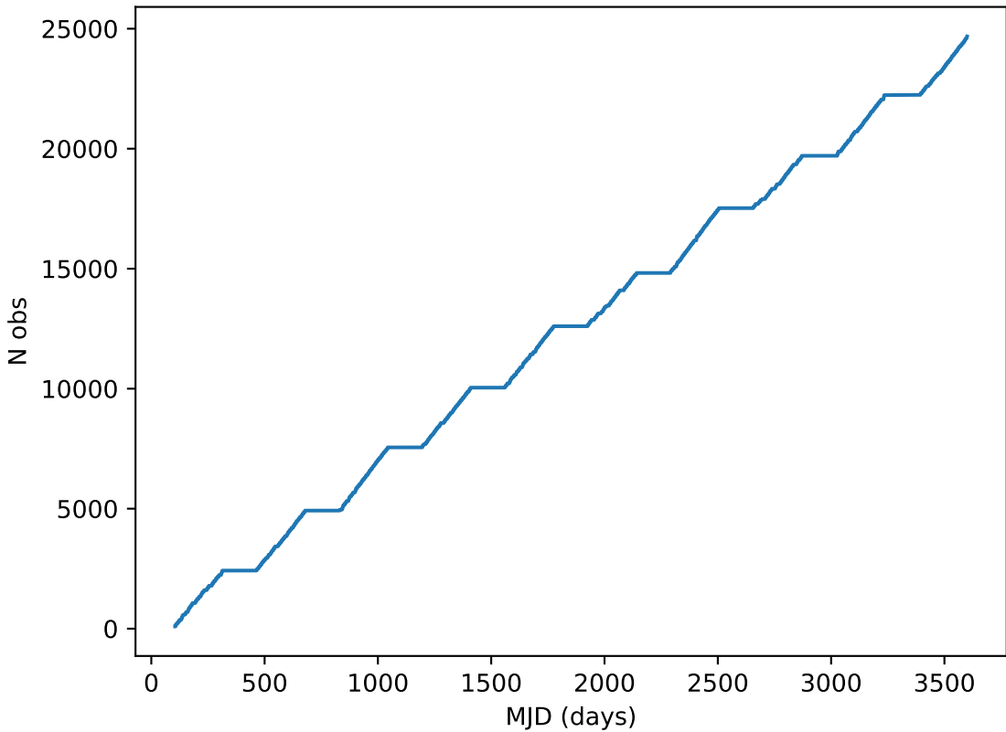
no_magell_roll_v3.4_10yrs all bands: DD:EDFS Cumulative NVisits
