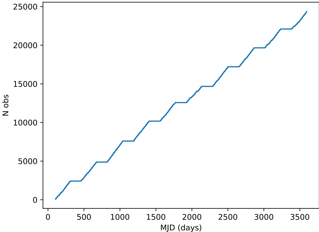
no_magell_roll_v3.4_10yrs all bands: DD:ECDFS Cumulative NVisits
