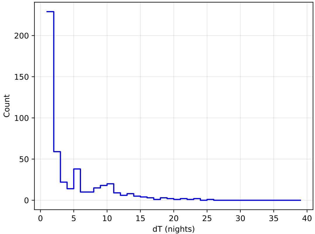
no_magell_roll_v3.4_10yrs all bands: DD: COSMOS Delta Nights Histogram
