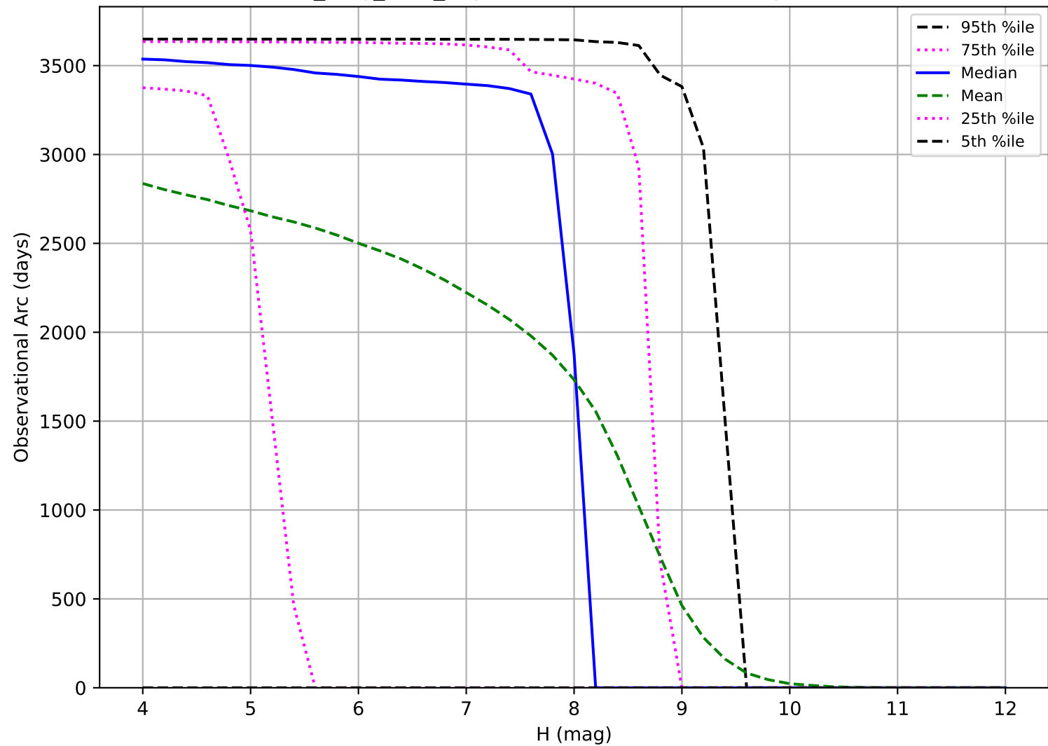
no_long_v3.4_10yrs: Observational Arc Length TNO
