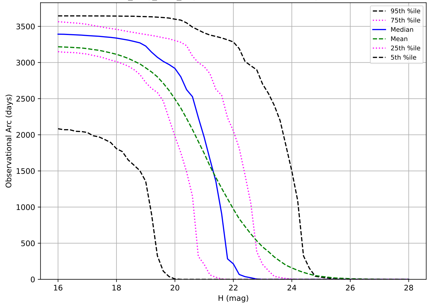
no_long_v3.4_10yrs: Observational Arc Length PHA
