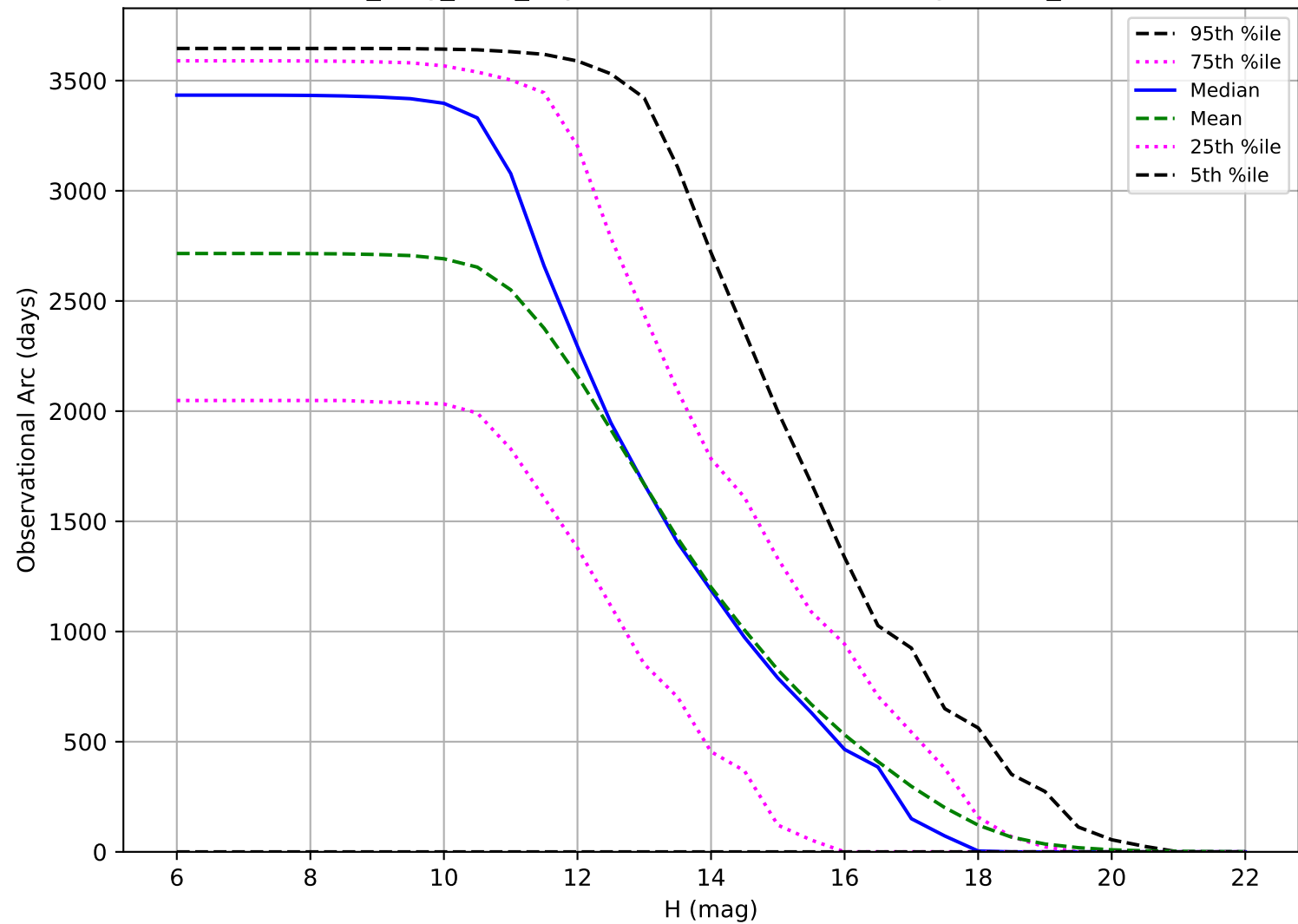
no_long_v3.4_10yrs: Observational Arc Length OCC_r5
