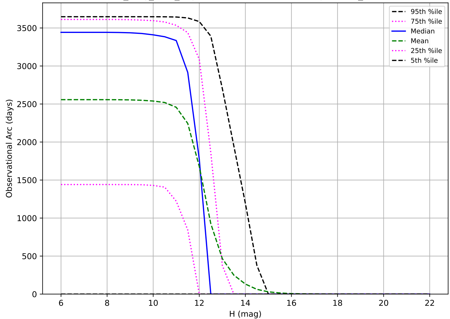
no_long_v3.4_10yrs: Observational Arc Length OCC_r20
