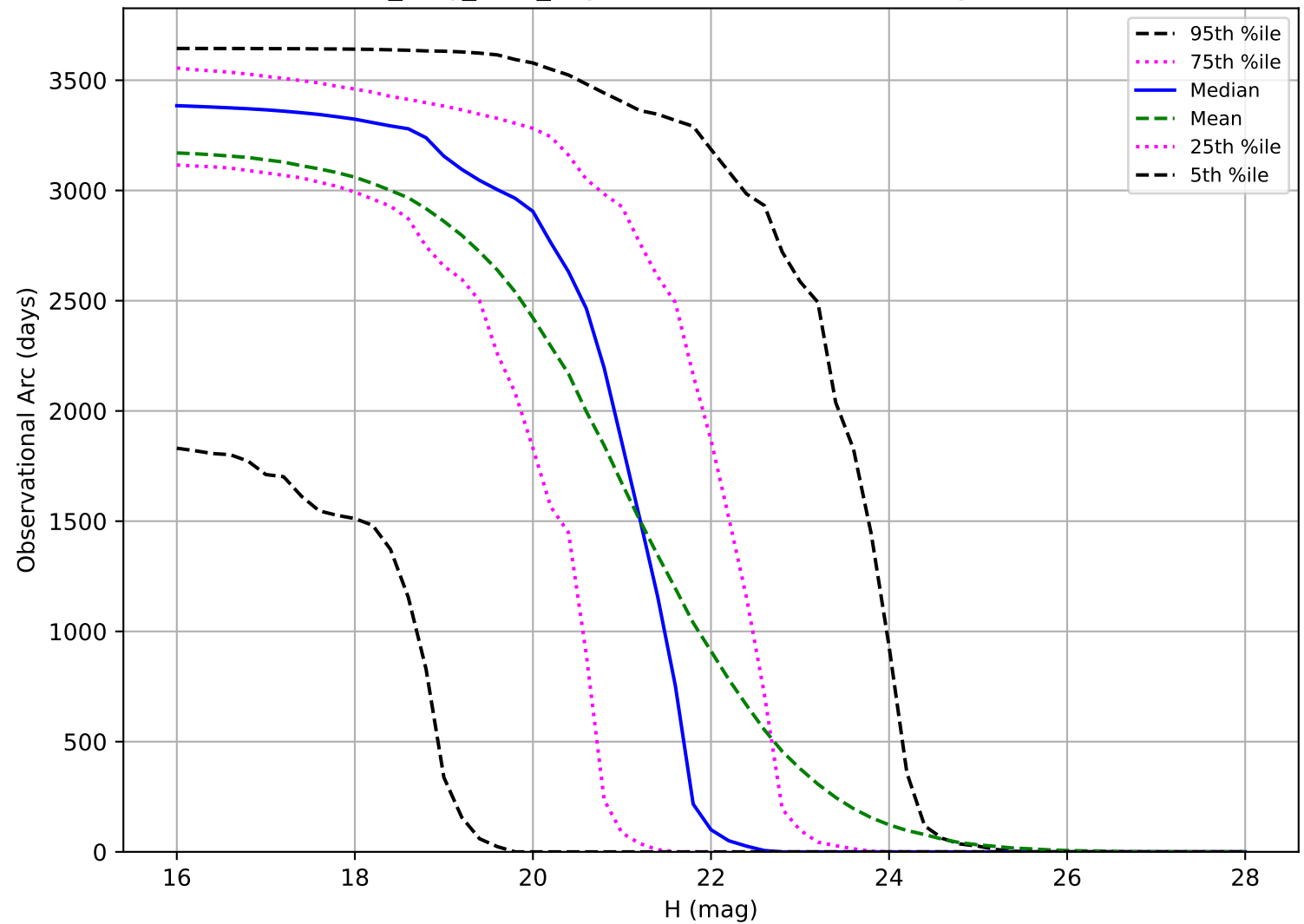
no_long_v3.4_10yrs: Observational Arc Length NEO
