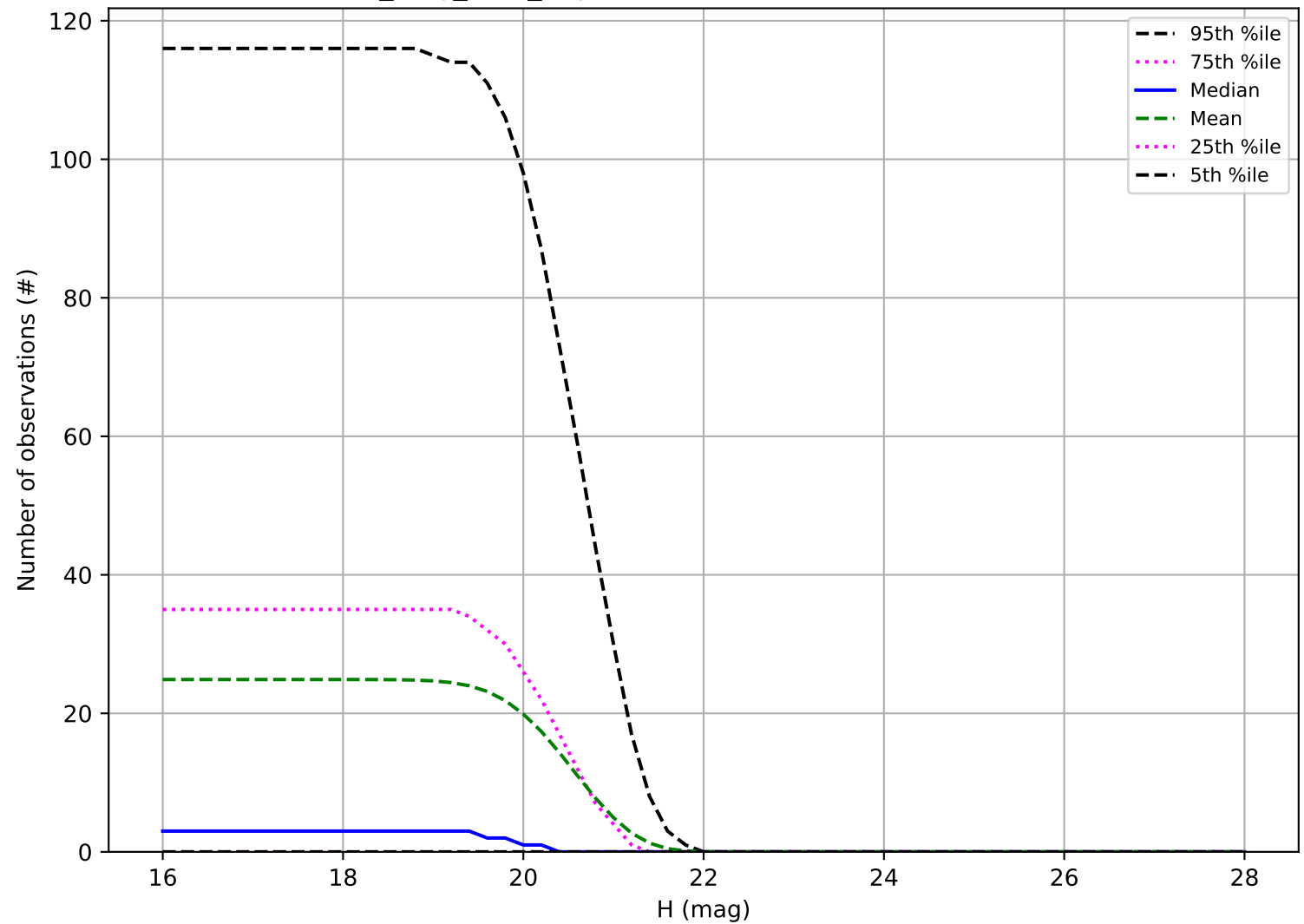
no_long_v3.4_10yrs: Number of observations Vatira
