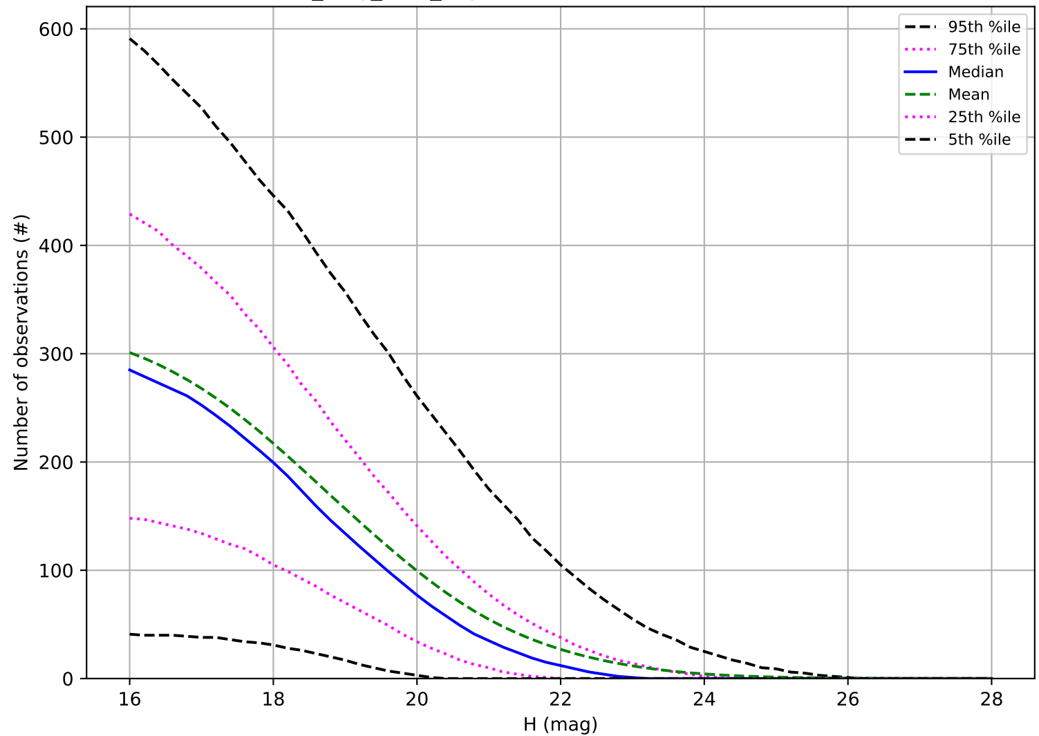
no_long_v3.4_10yrs: Number of observations PHA
