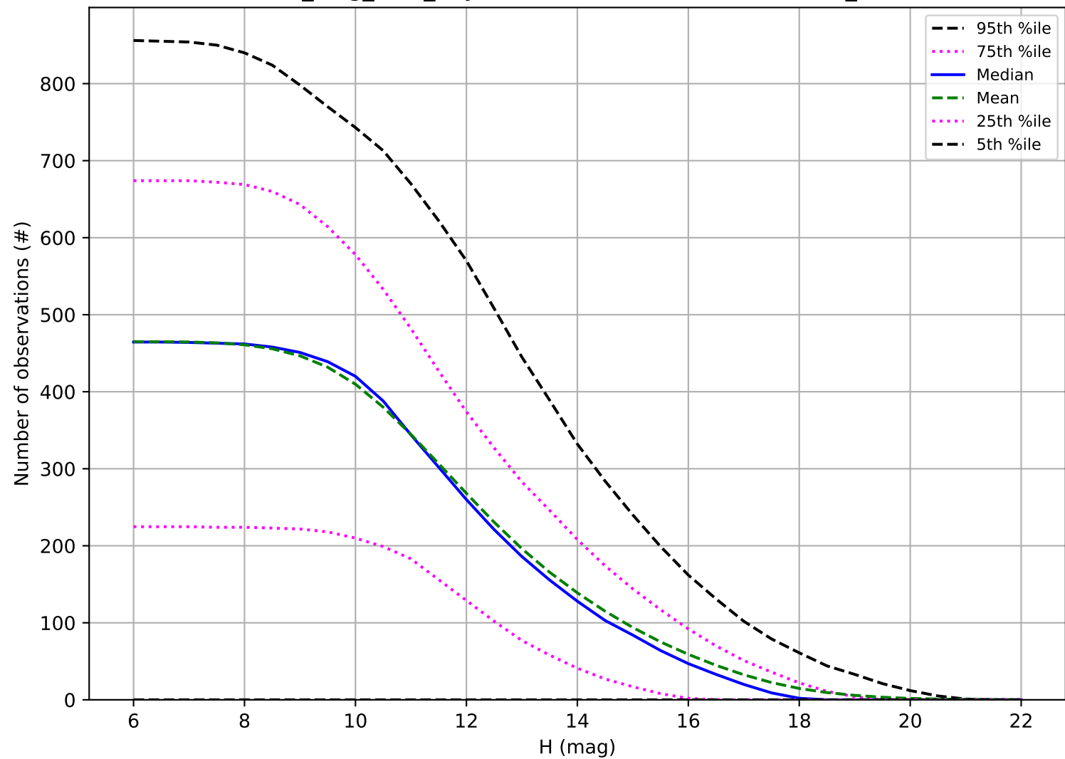
no_long_v3.4_10yrs: Number of observations OCC_r5
