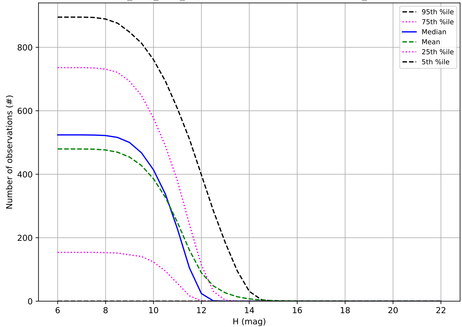
no_long_v3.4_10yrs: Number of observations OCC_r20
