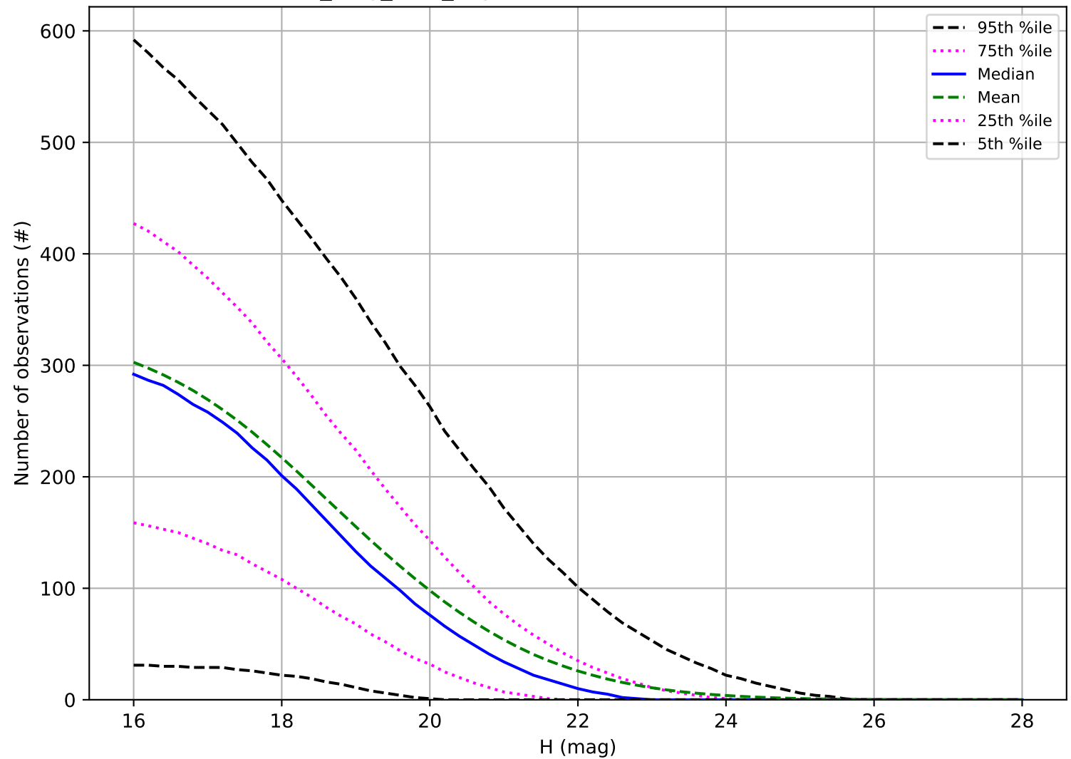
no_long_v3.4_10yrs: Number of observations NEO
