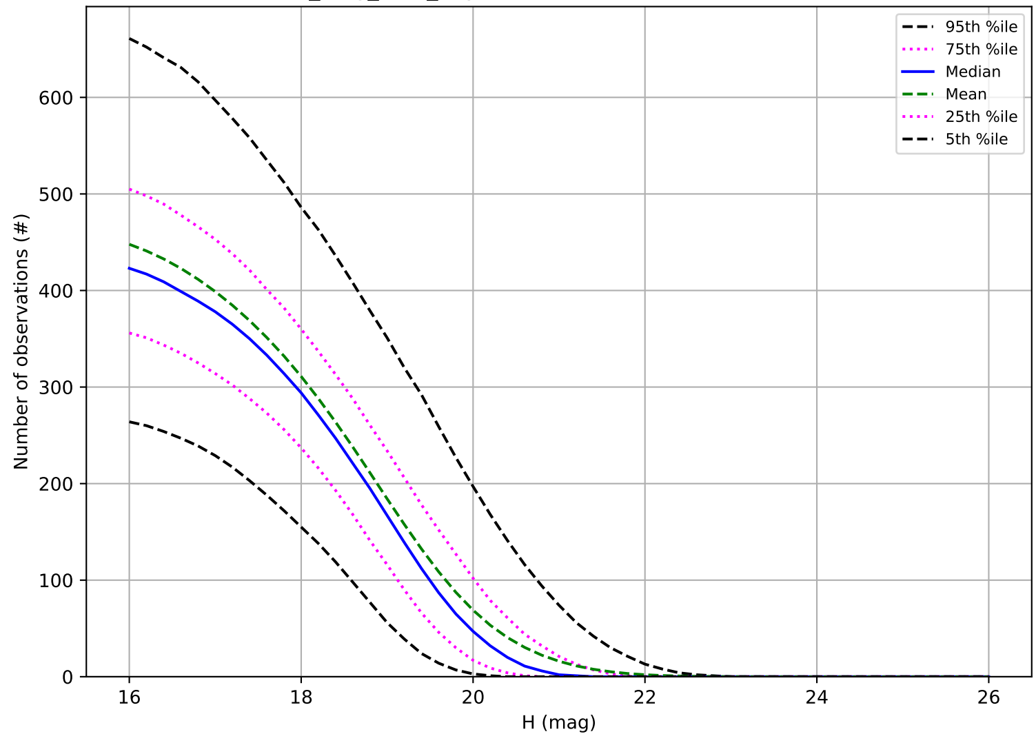
no_long_v3.4_10yrs: Number of observations MBA
