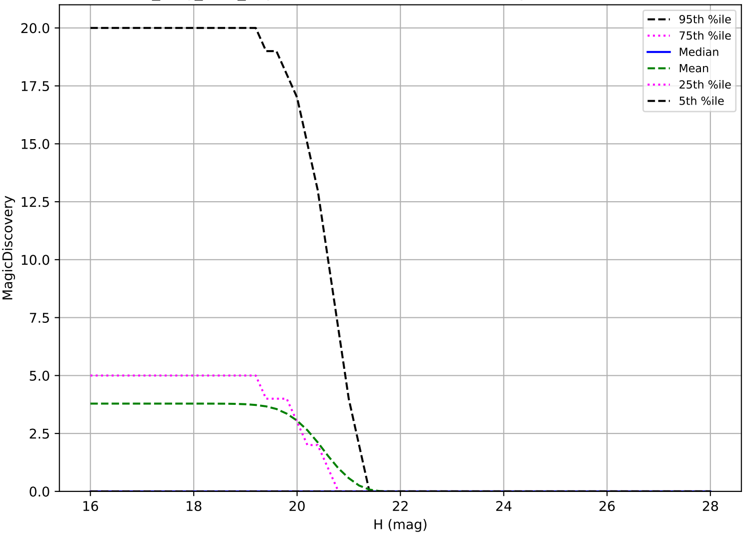
no_long_v3.4_10yrs: Vatira 6 detections in 60 nights detection loss
