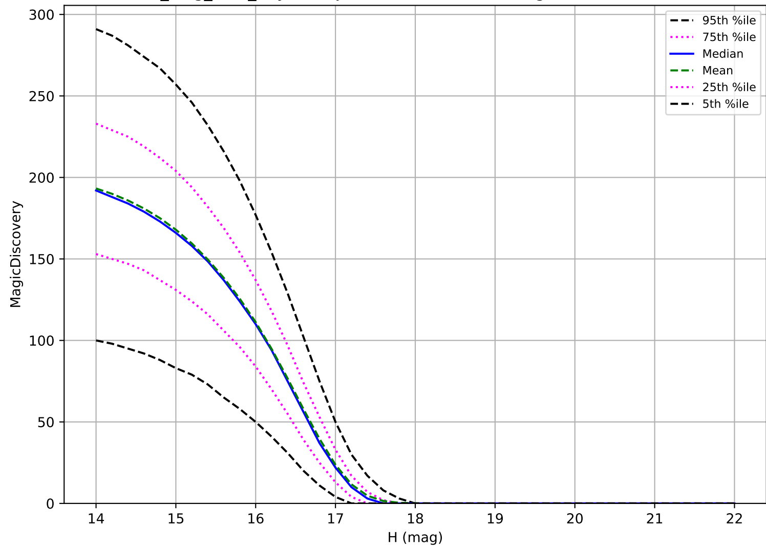
no_long_v3.4_10yrs: Trojan 6 detections in 60 nights detection loss
