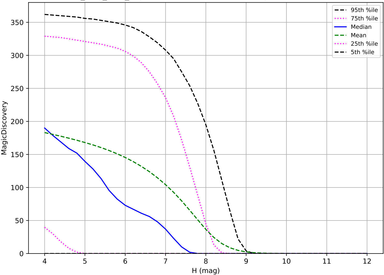
no_long_v3.4_10yrs: TNO 6 detections in 60 nights detection loss
