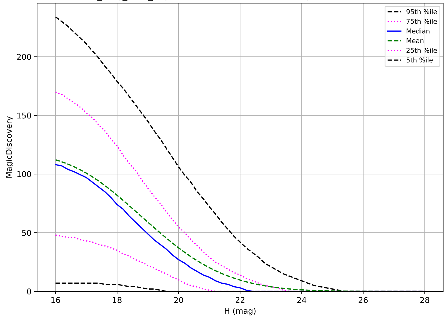
no_long_v3.4_10yrs: PHA 6 detections in 60 nights detection loss
