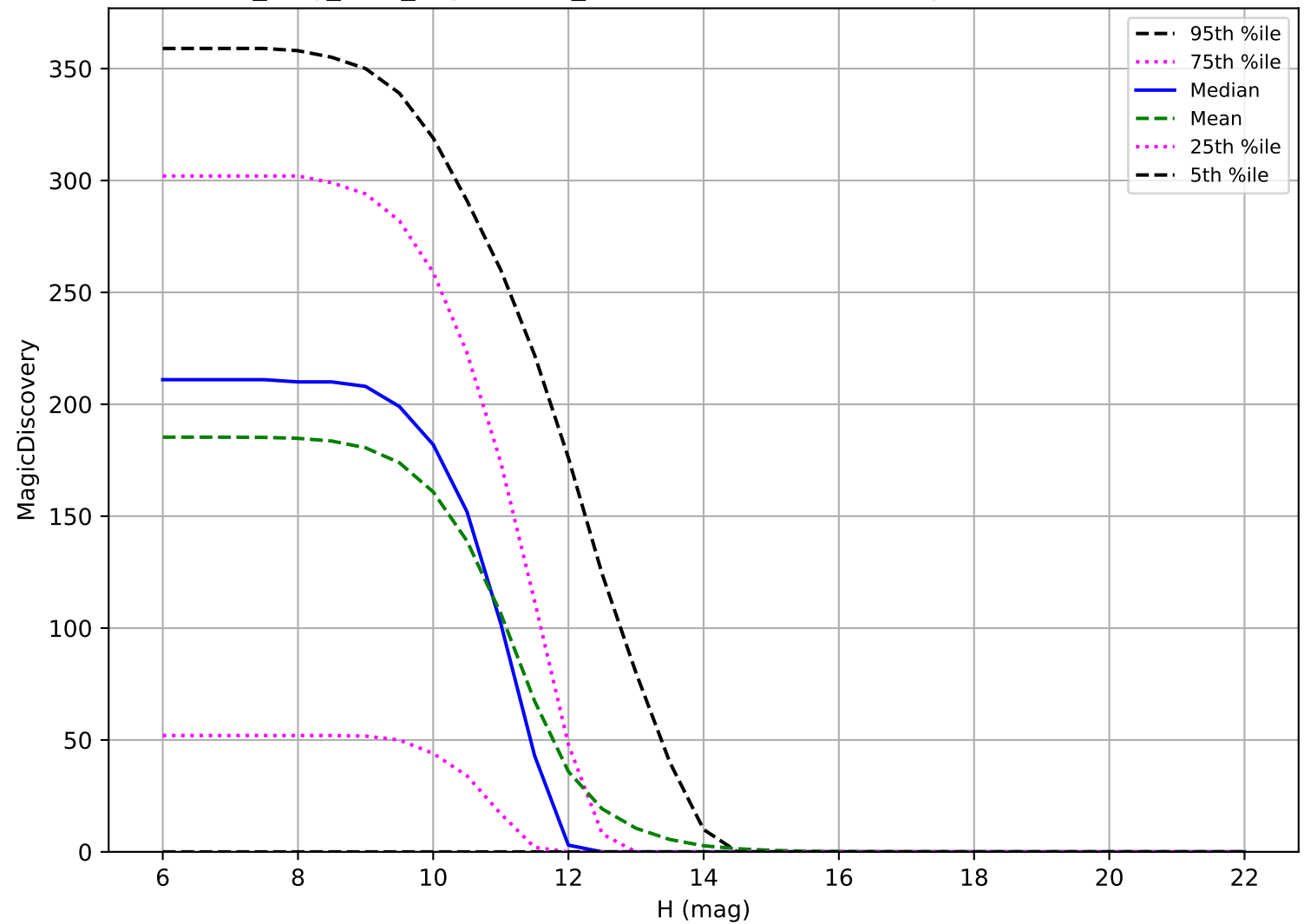
no_long_v3.4_10yrs: OCC_r20 6 detections in 60 nights detection loss
