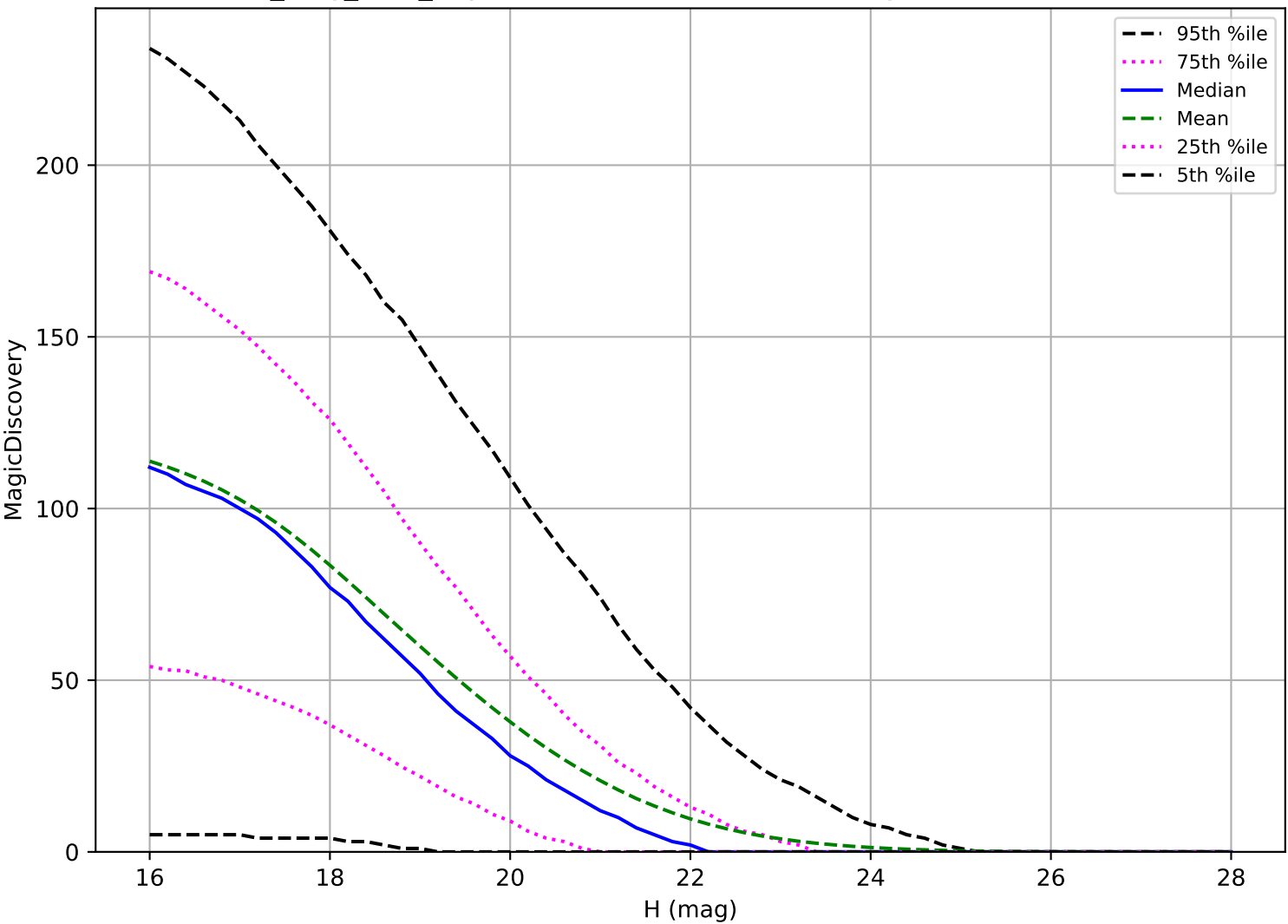
no_long_v3.4_10yrs: NEO 6 detections in 60 nights detection loss
