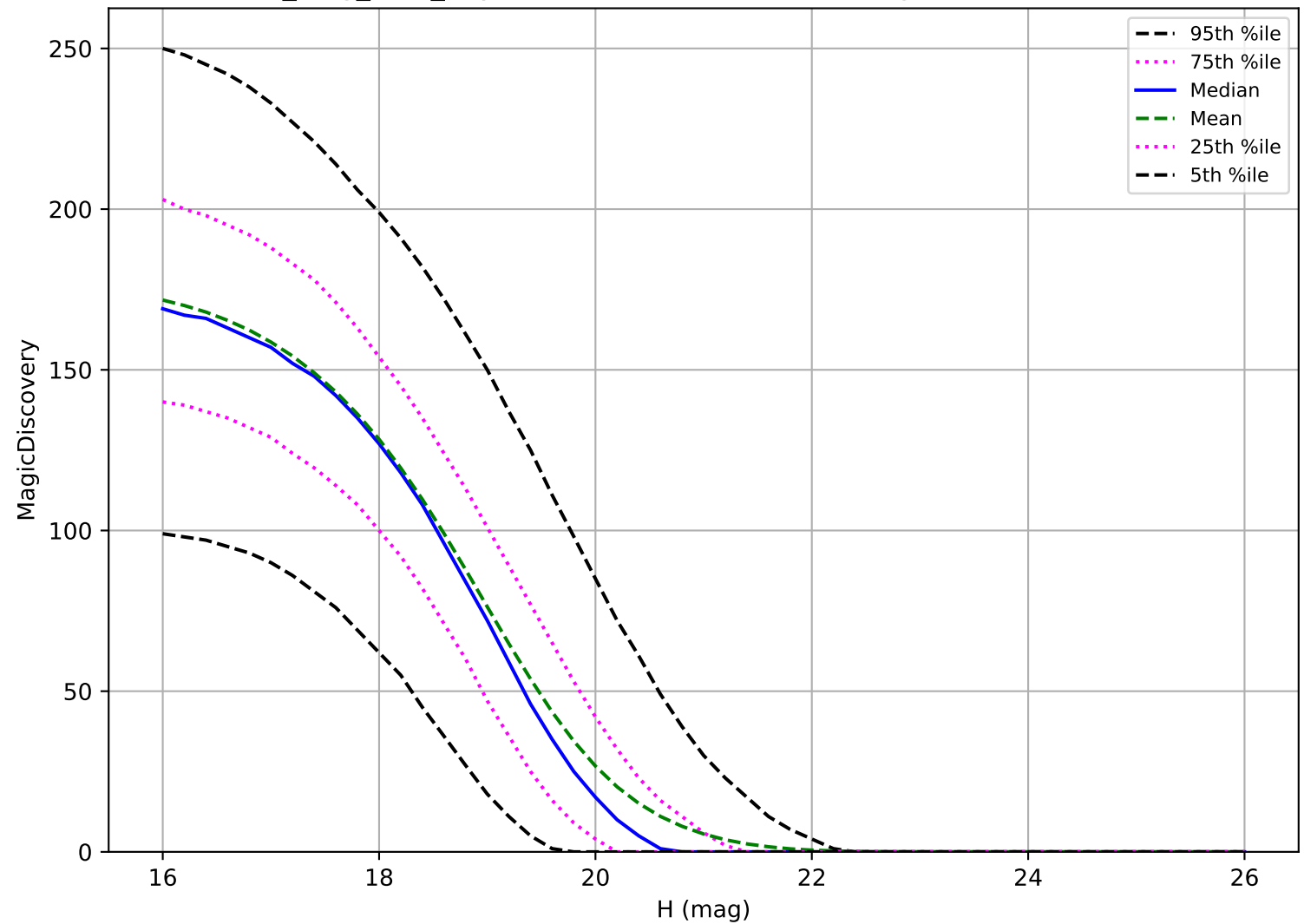
no_long_v3.4_10yrs: MBA 6 detections in 60 nights detection loss
