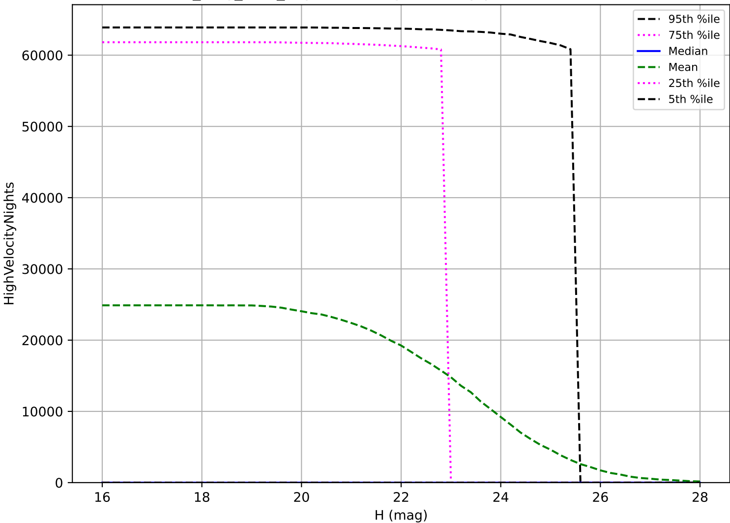
no_long_v3.4_10yrs: PHA High velocity pair detection loss
