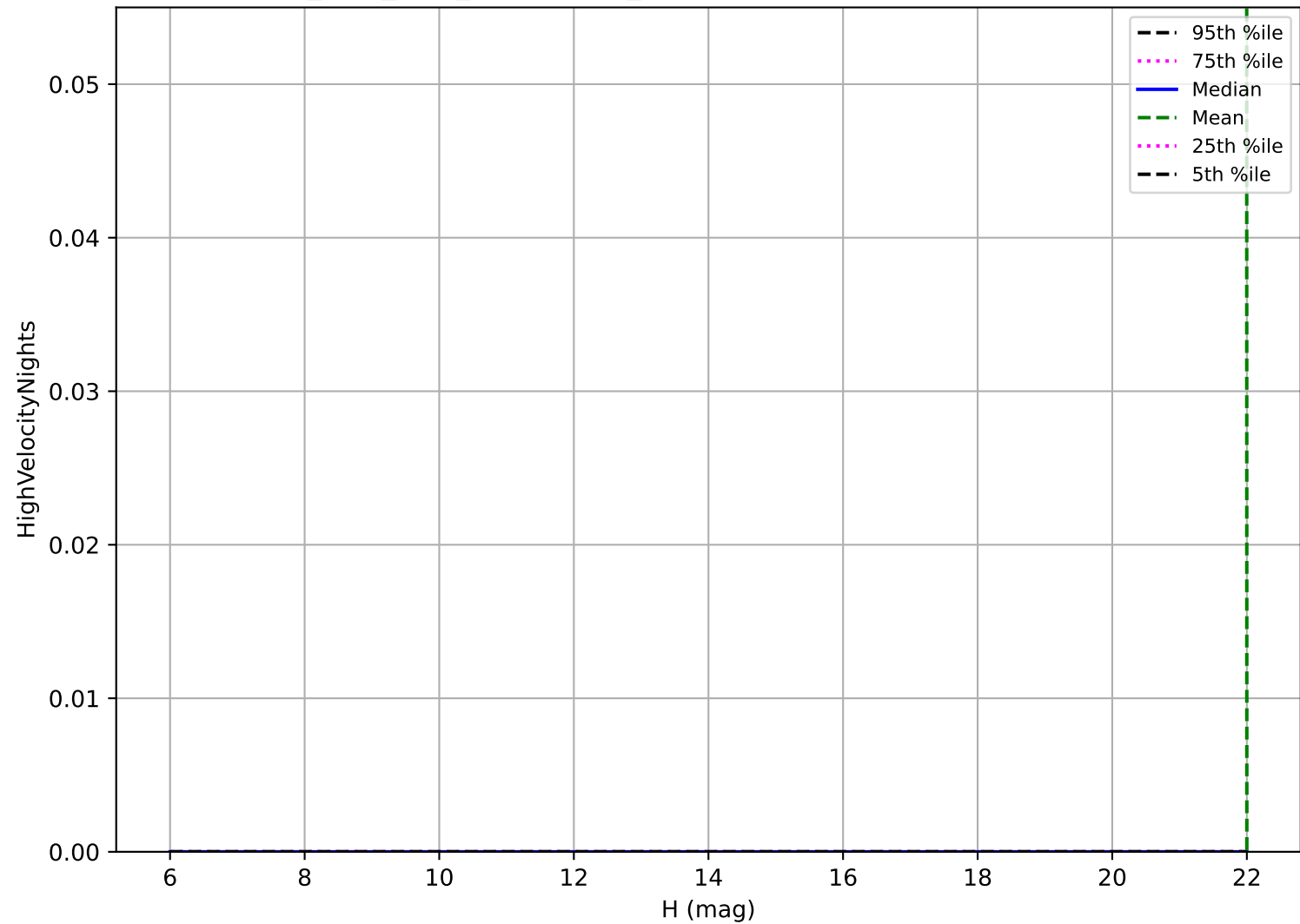
no_long_v3.4_10yrs: OCC_r20 High velocity pair detection loss
