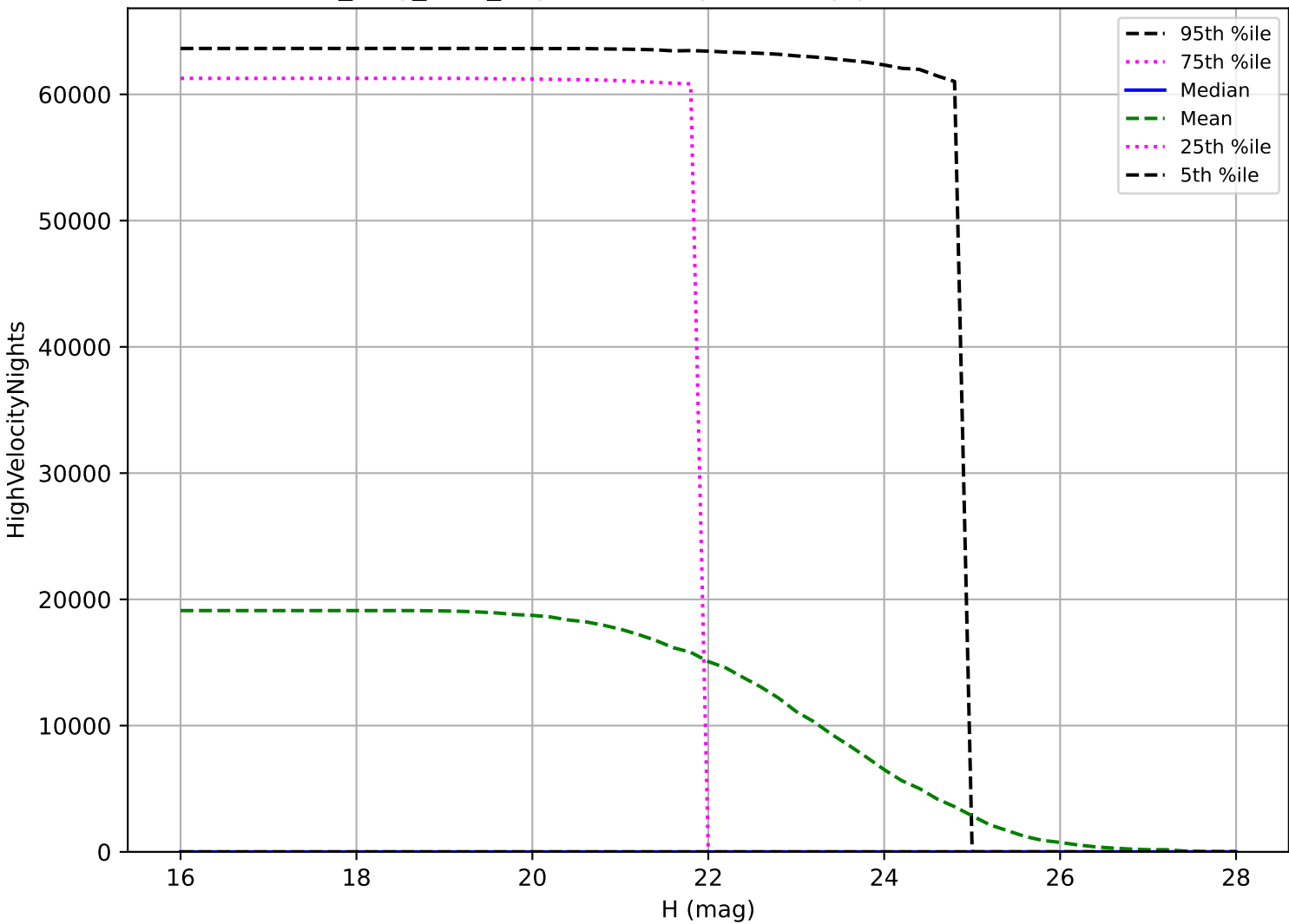
no_long_v3.4_10yrs: NEO High velocity pair detection loss
