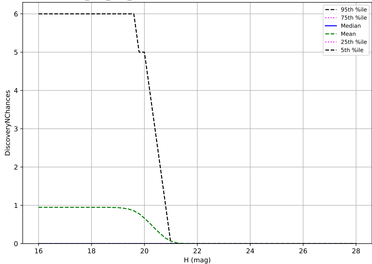
no_long_v3.4_10yrs: Vatira 3 pairs in 15 nights detection loss
