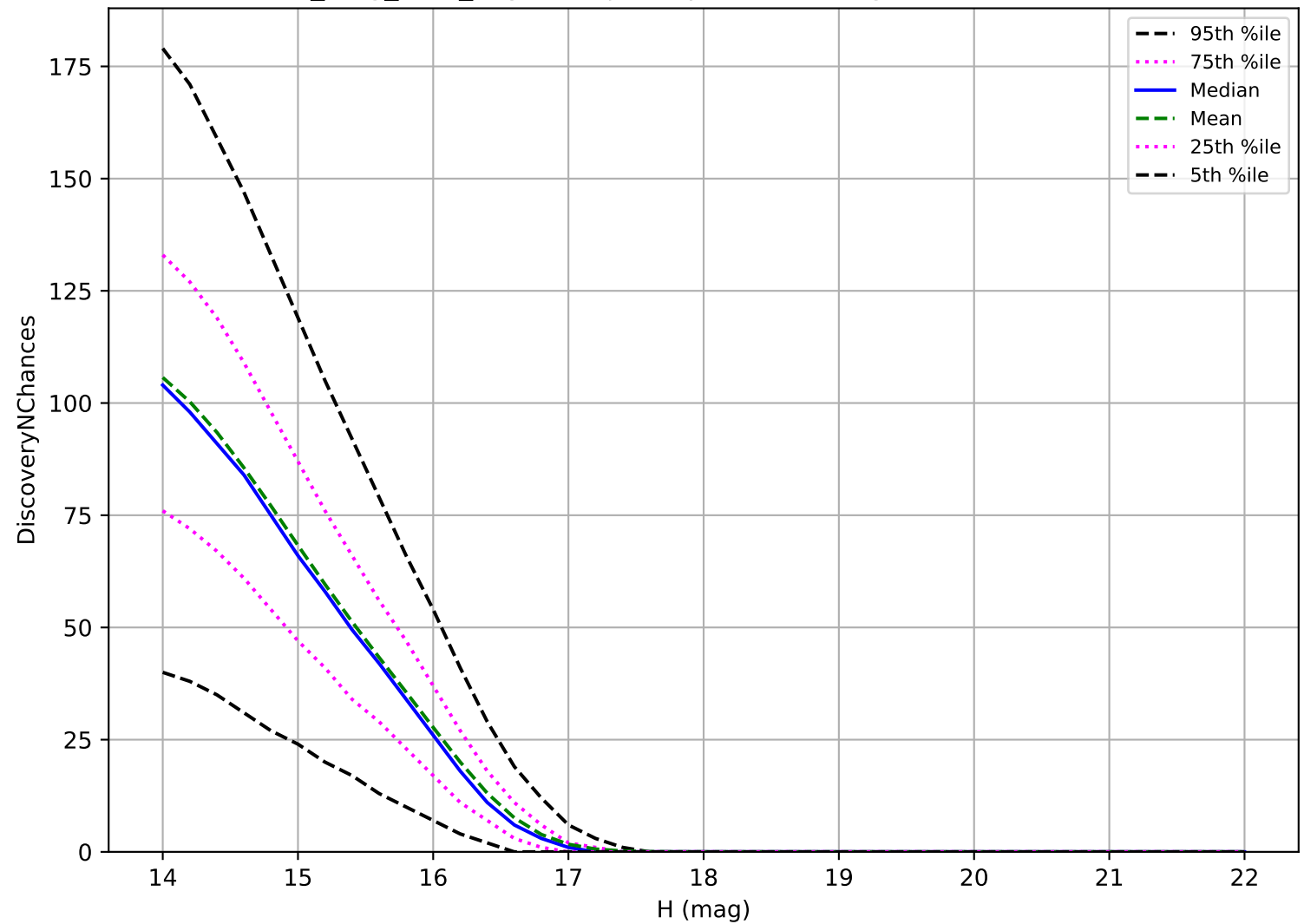
no_long_v3.4_10yrs: Trojan 3 pairs in 15 nights detection loss
