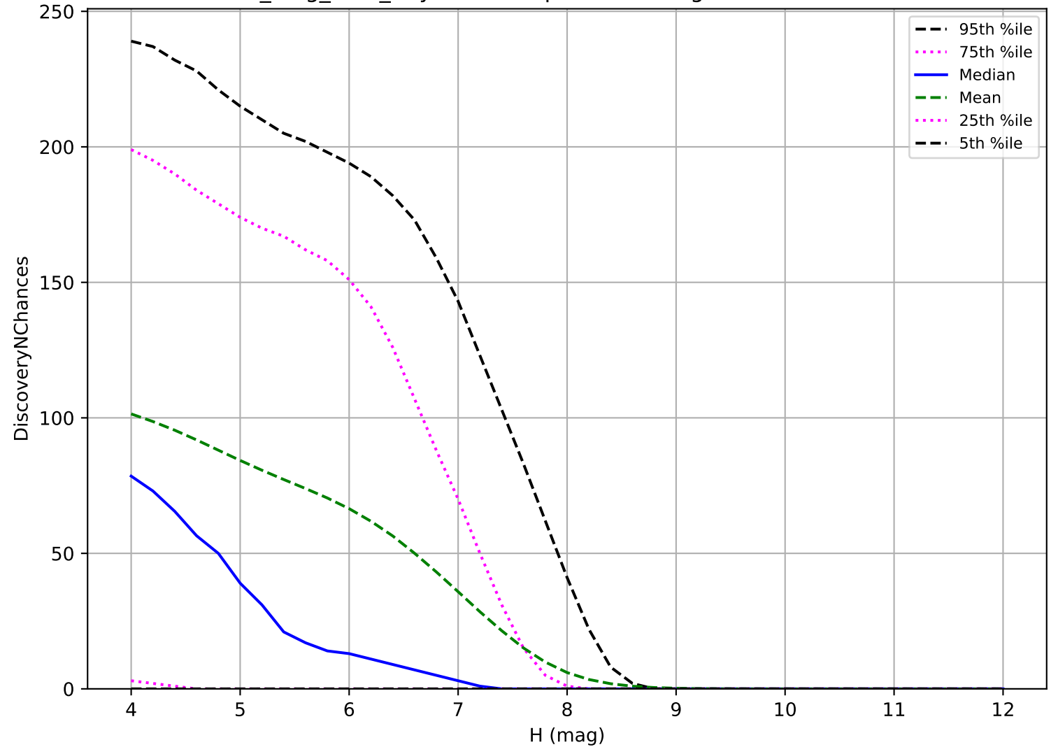
no_long_v3.4_10yrs: TNO 3 pairs in 15 nights detection loss
