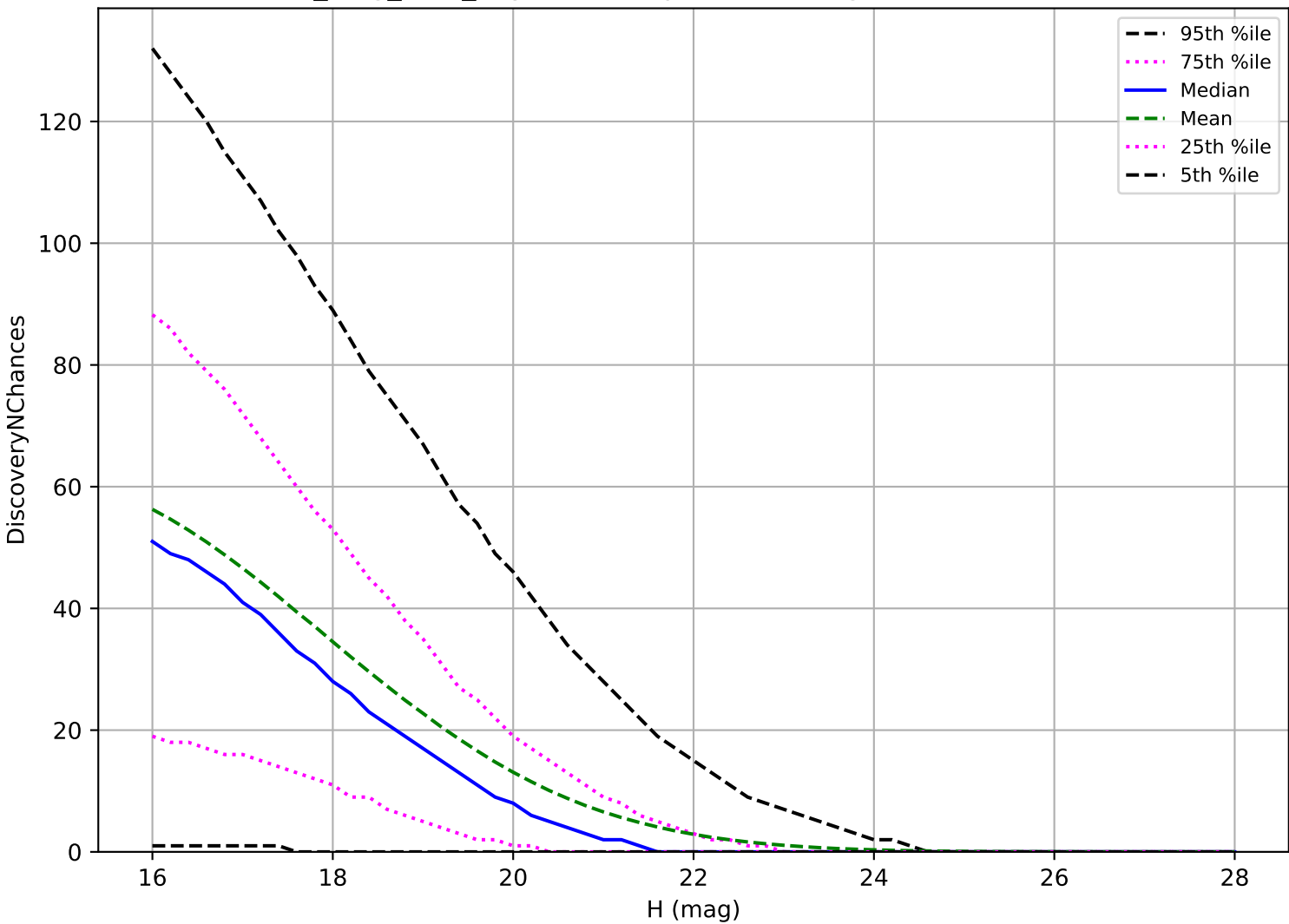
no_long_v3.4_10yrs: PHA 3 pairs in 15 nights detection loss
