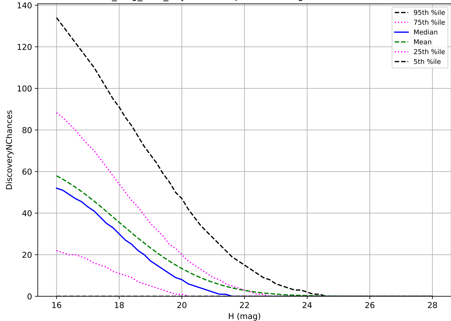
no_long_v3.4_10yrs: NEO 3 pairs in 15 nights detection loss
